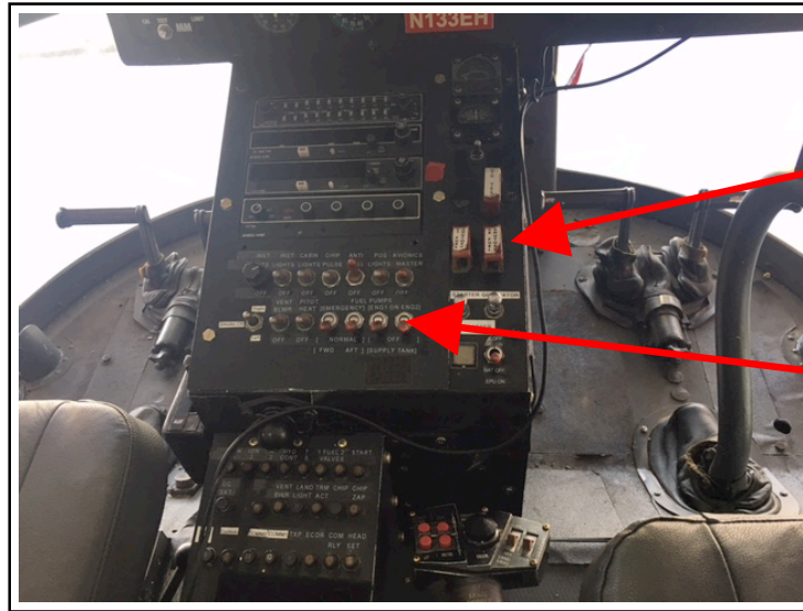
Fuel Pump Switches x4 – down = off
